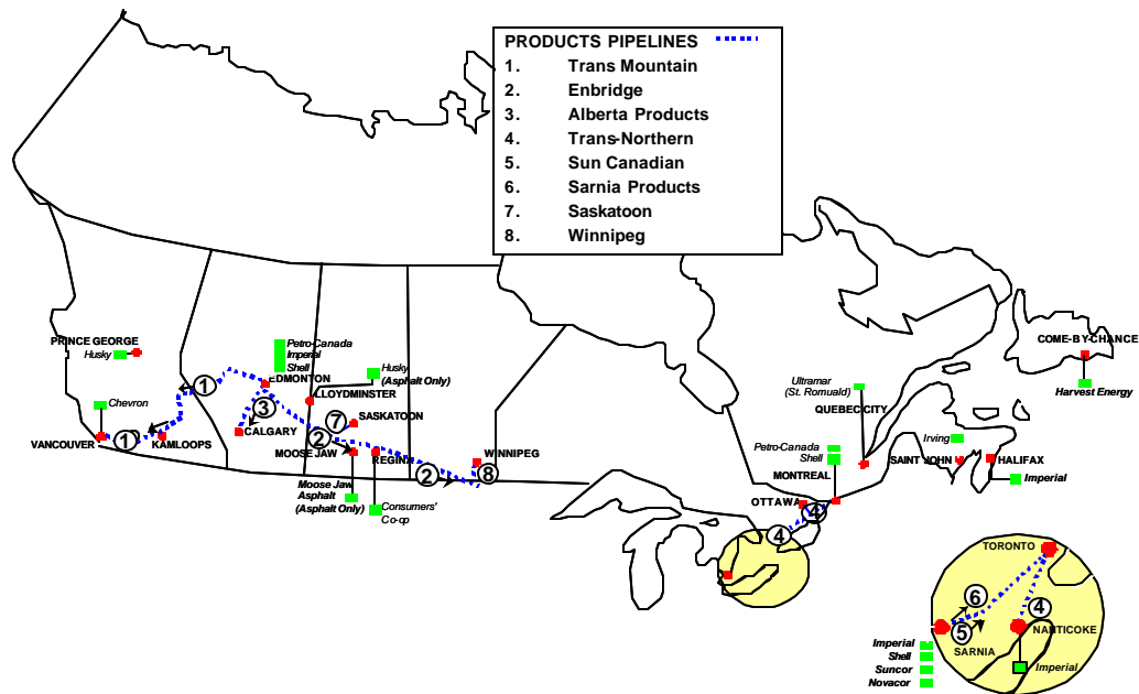
Figure 4: Refined product pipelines in Canada
